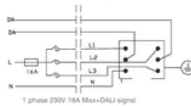
3 circuit DALI track system
